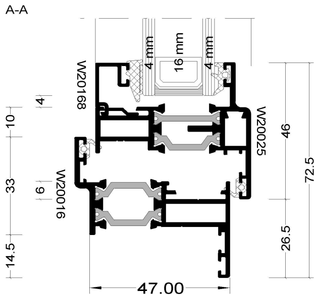
Equal leg outer-frame with sash - Door
