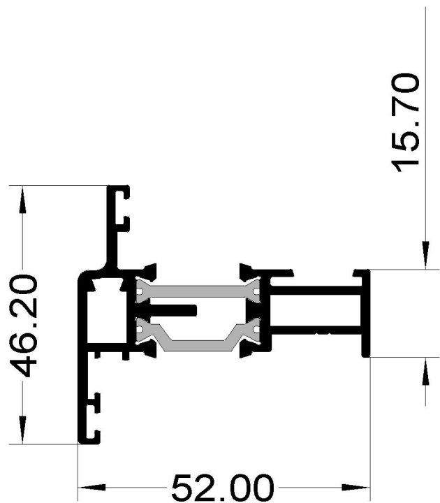
W20025 - Window sash
