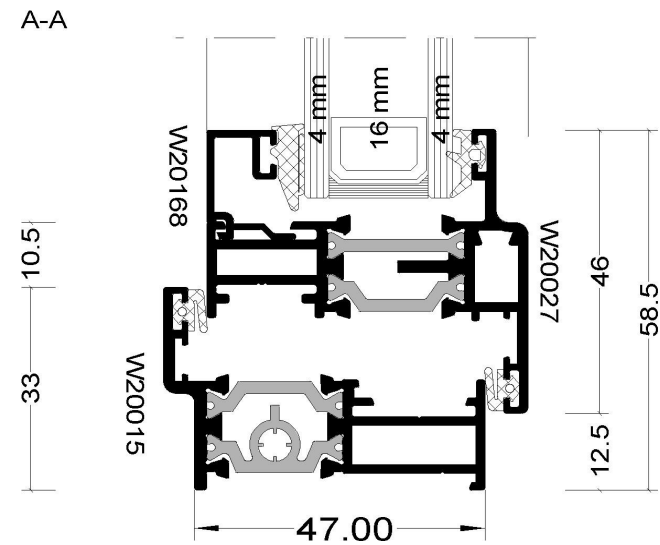
Equal leg outer-frame with sash - Door
