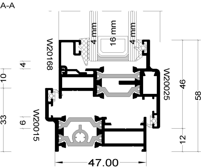
Equal leg outer-frame with sash - Window
